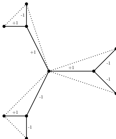
Figure 2: The ball of radius two centered at x in a realization of the random graph (T, x) .
