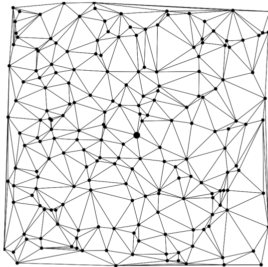
Figure 3: An approximate Poisson-Delaunay triangulation
