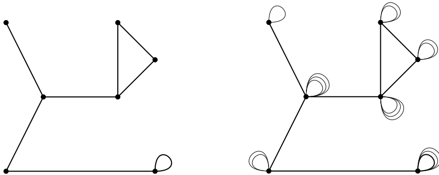
Figure 1: The stationary distribution m(x) = \deg(x) / \sum \deg(y) of a finite graph does not change when one adds \deg(x) loops at each vertex x . For general stationary random graphs this process does not affect stationarity.
