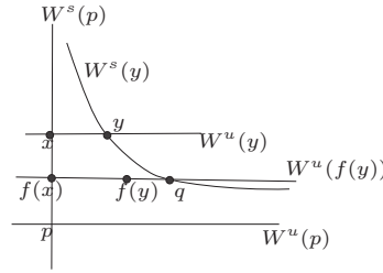
FIGURE 3. Invariant stable II
