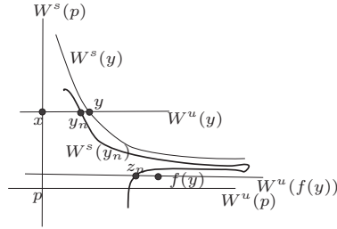
FIGURE 4. Invariant stable III
