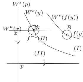
FIGURE 2. Invariant stable I
